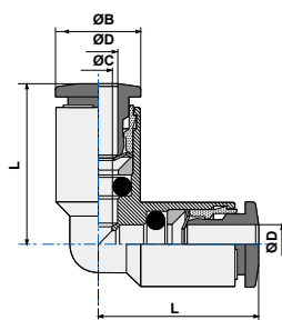
ART. 04SS L型 Elbow connector
